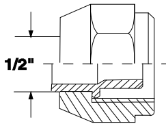
3/4-16 Thread No. 8 FEMALE O-RING
