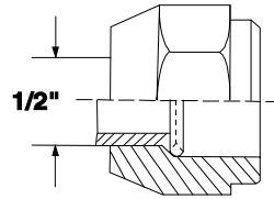
3/4-16 Thread NO. 8 FEMALE FLARE
