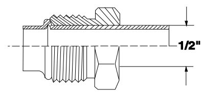
3/4-18 Thread No. 8 MALE O-RING
