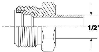
3/4-16 Thread No. 8 MALE INSERT O-RING
