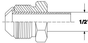
3/4-16 Thread NO. 8 MALE FLARE
